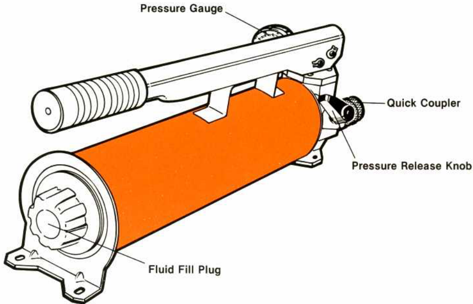
2 Stage Hydraulic Hand Pump For Model 402 & 401 Kits
